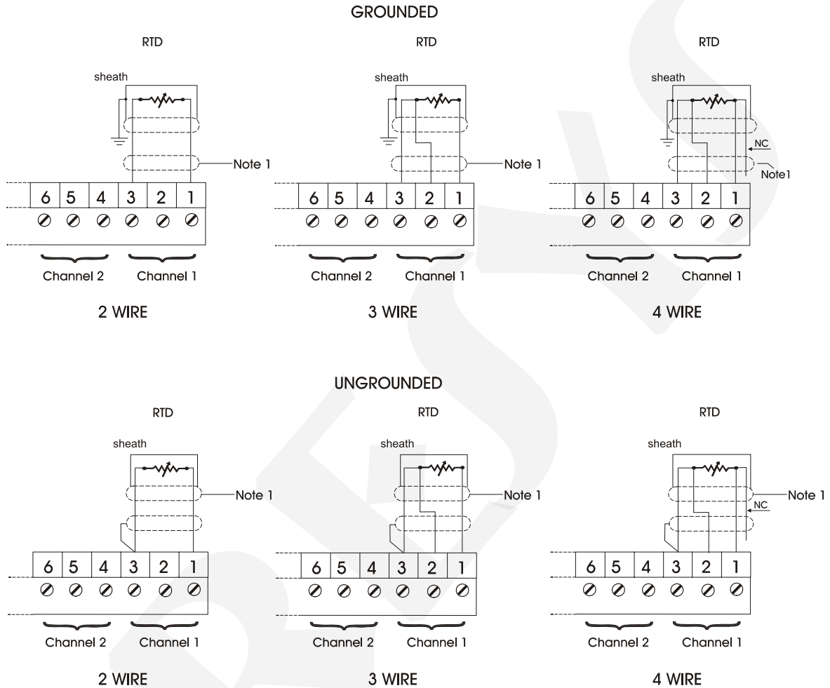
Fig. 6 – RTD Connection
