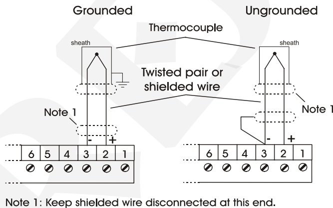
Fig. 5 - Thermocouple Connection
