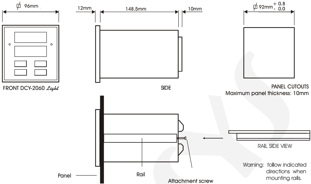
Fig. 3 - Dimensional drawing, panel mounting cutout and side view for DCY-2060 Light controllers
