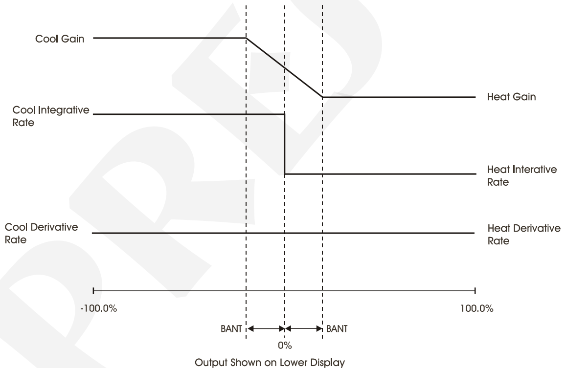
Fig. 27 - PID parameter variation in the heating-cooling transition
