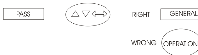
Fig. 12 – Password system
