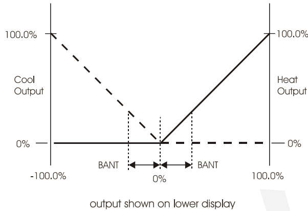
Fig. 26 - Heating-cooling output transition
